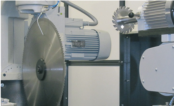
Profile machining centre SBZ 630
