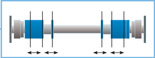
Fig. 20: Saw shaft with up to four moving telescopic saw bushes
