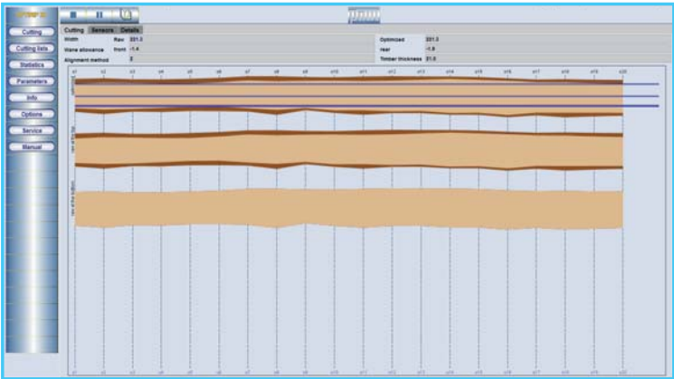
Fig. 5: Screenshot of the ripping pattern
