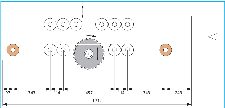
Fig. 19: Minimum roller configuration of an M34
