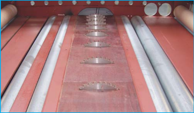
Fig. 5: Insert table with rip saws and bottom feed rollers
