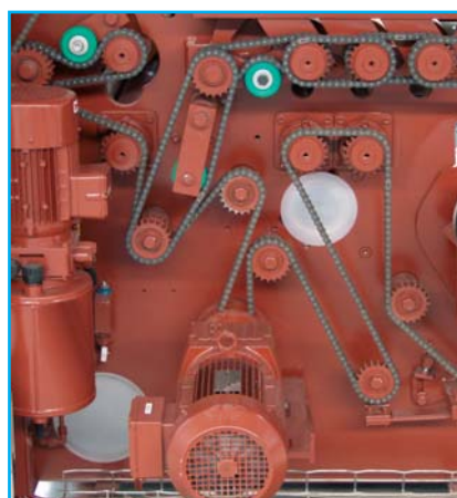
Fig. 17: Feed drive via chains
