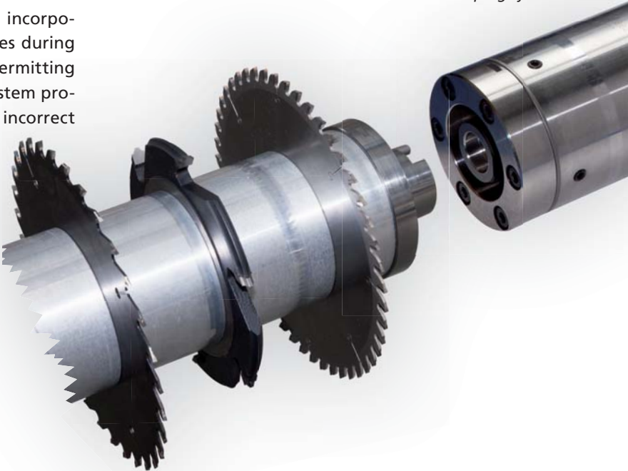
Fig. 13: HSK saw shaft clamping system
