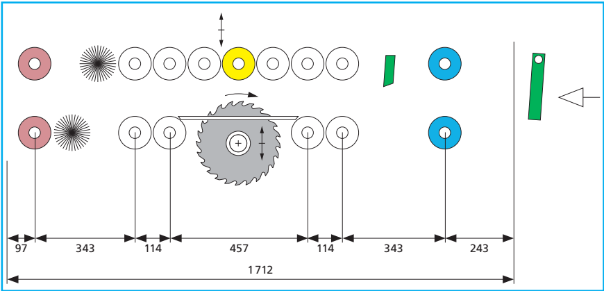
Fig. 20: Maximum roller configuration of an M34
